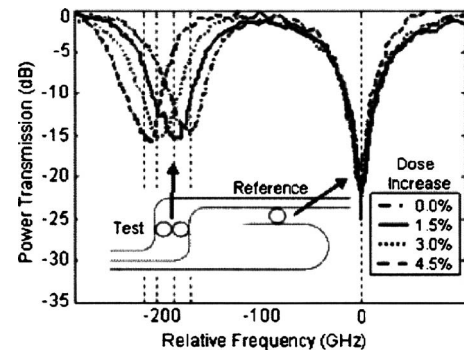
FIG. 2. Sample set of transmission spectra used for dose calibration experiments. Inset displays the device layout with a reference filter for each test filter. All frequencies are measured relative to the reference filter resonant frequency.
